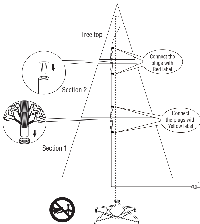
Fig. B - Tree and Light Assembly
